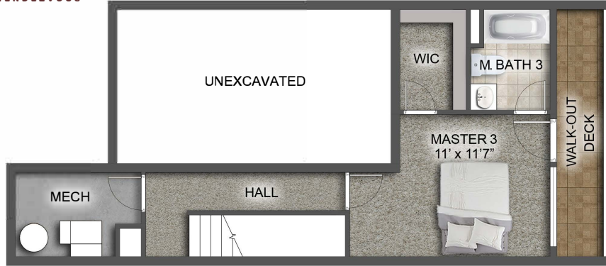
WALKOUT FLOOR PLAN
