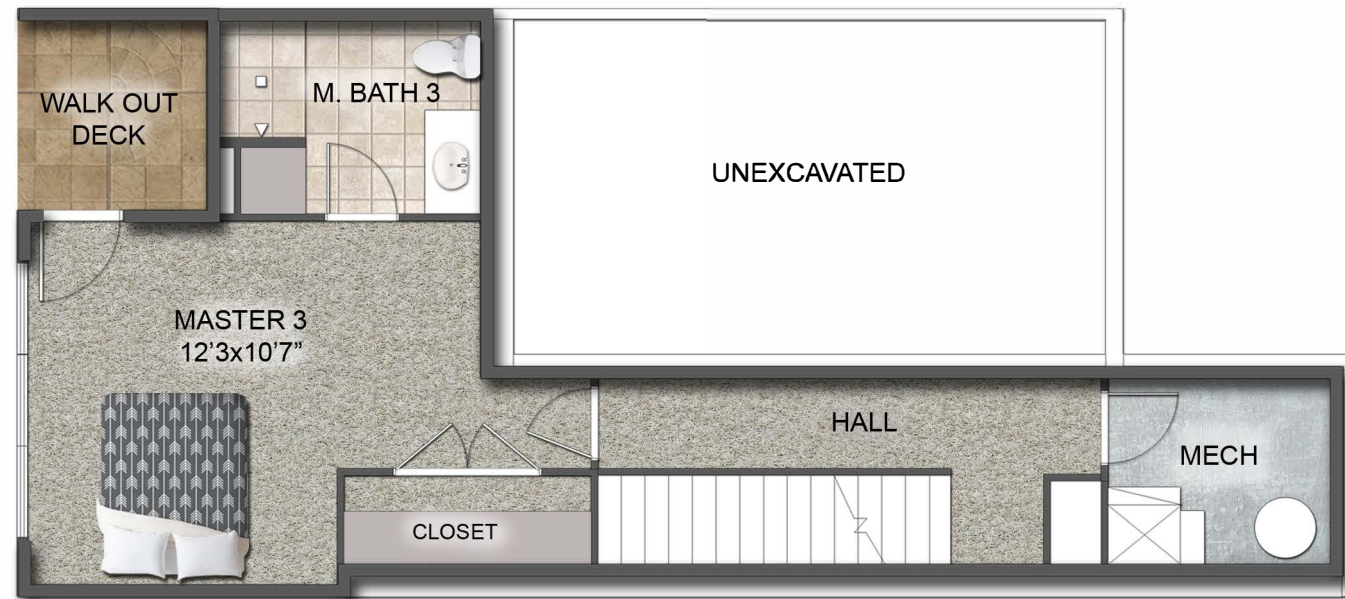
WALKOUT PLAN
