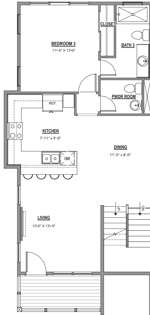
Plan B - Second Level
