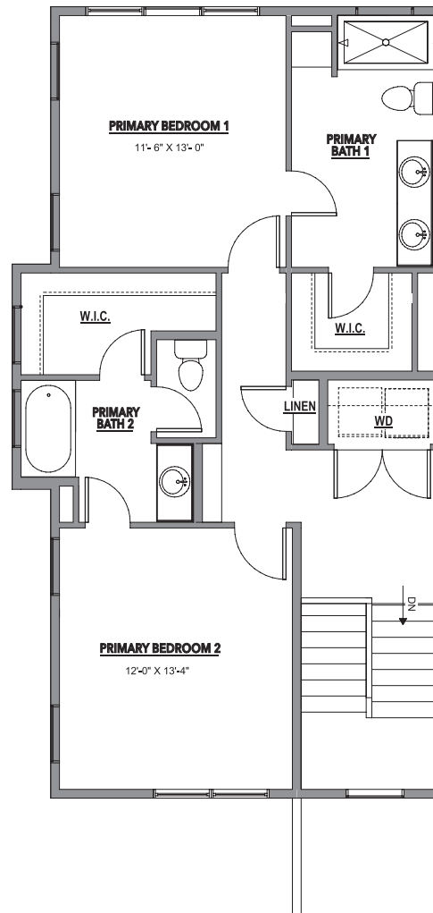
Plan B - Third Level
