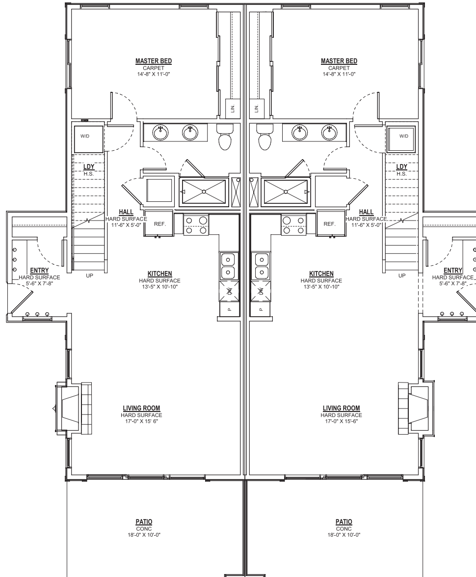
MAIN LEVEL FLOOR PLAN
